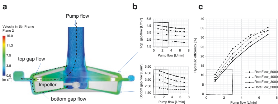
Fig. 8.2 Gap flow (panels a and b ) and hydraulic efficiency (panel c ) of rotary blood pumps
